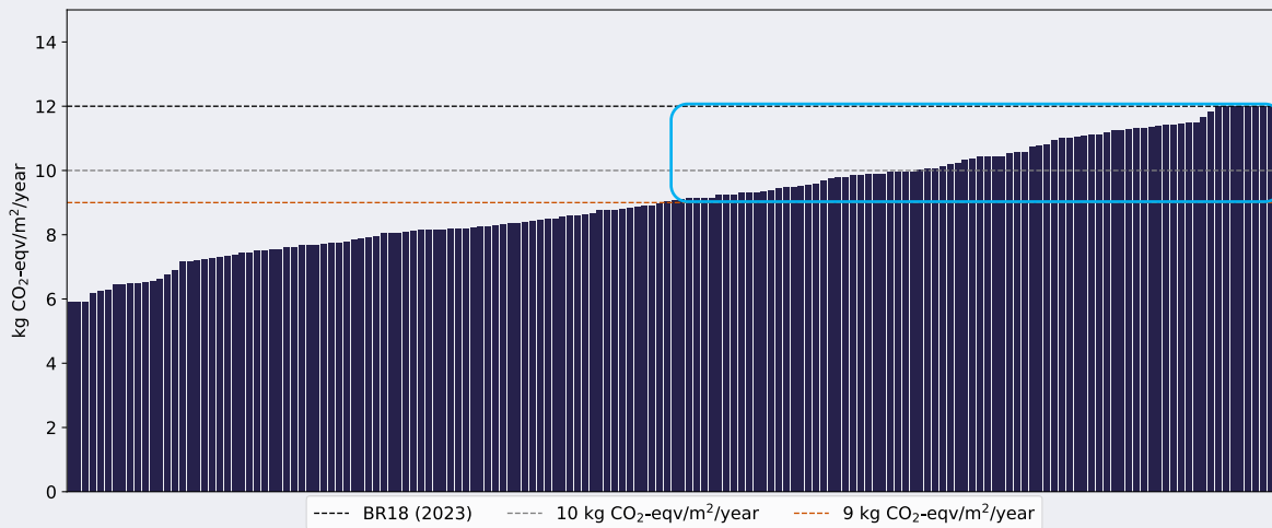
Figure 3. Illustration of the potential for reduction (blue box) of greenhouse gas emissions by tightening the limit value. The results are reported in kg CO 2 -eqv/m 2 /year over a reference study period of 50 years.
